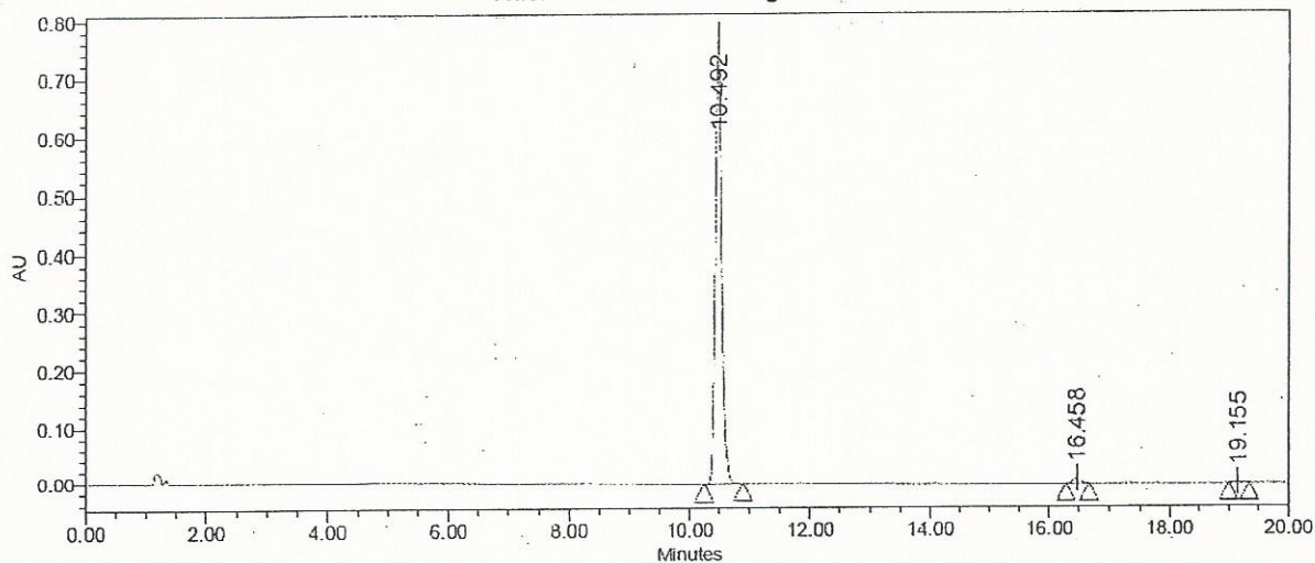
Auto-Scaled Chromatogram
